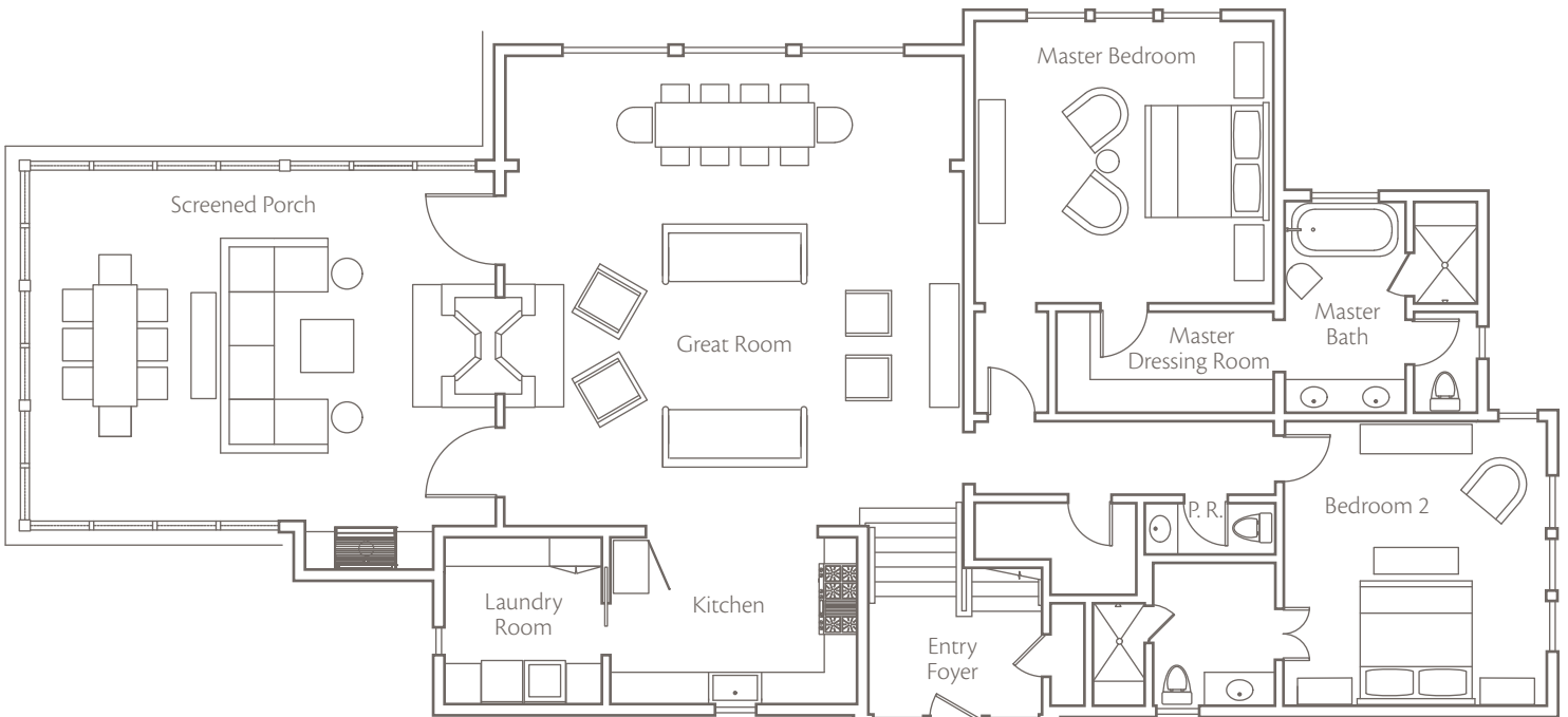
FIRST FLOOR
